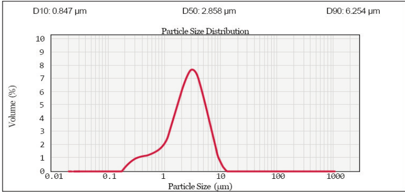
Ceroxid HD W2535 PSD laser particle size distribution analyzer
